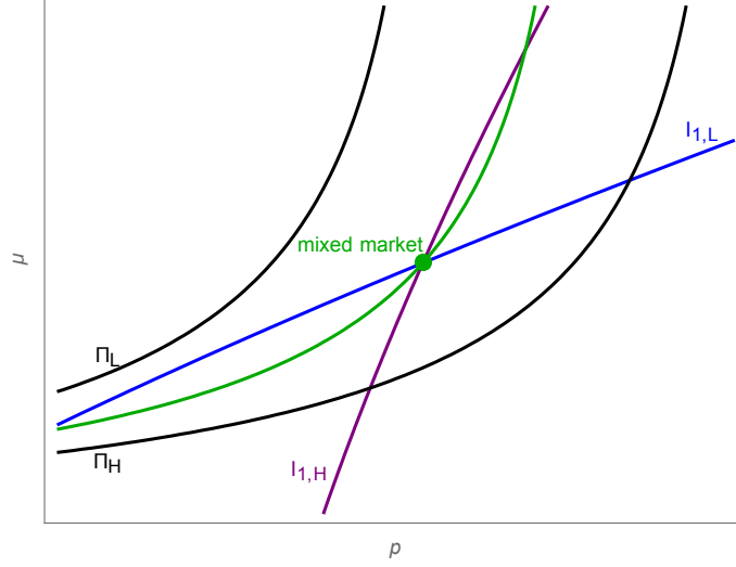
Figure 3: Cream-skimming deviation in the single-application case.
