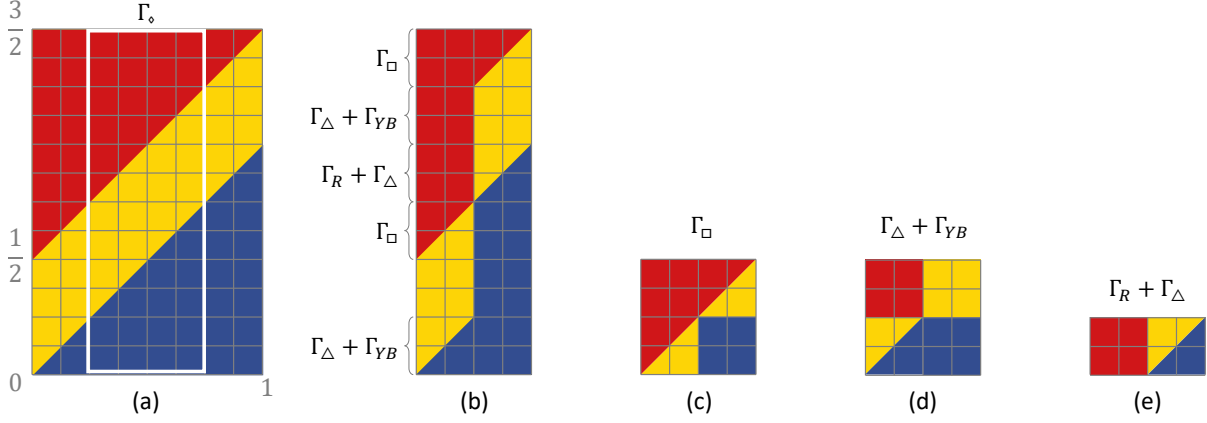
Figure 10: Recursive conversation for game \Gamma_{\diamond}^{\ell} , with \ell = 3/2
