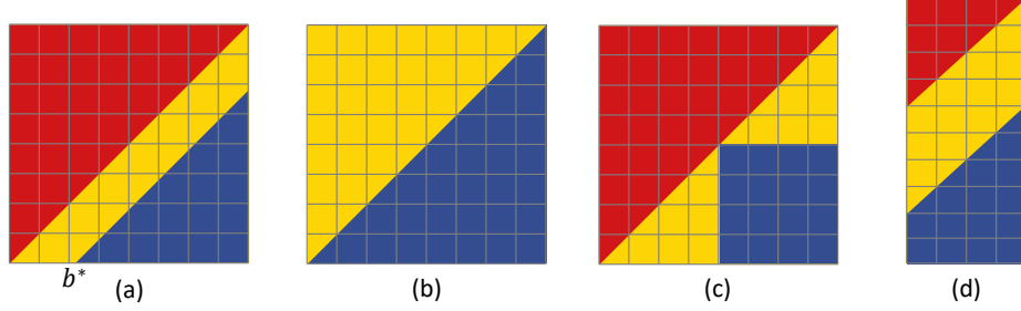
Figure 12: Biased observer model (a) and continuation games (b)-(d)
