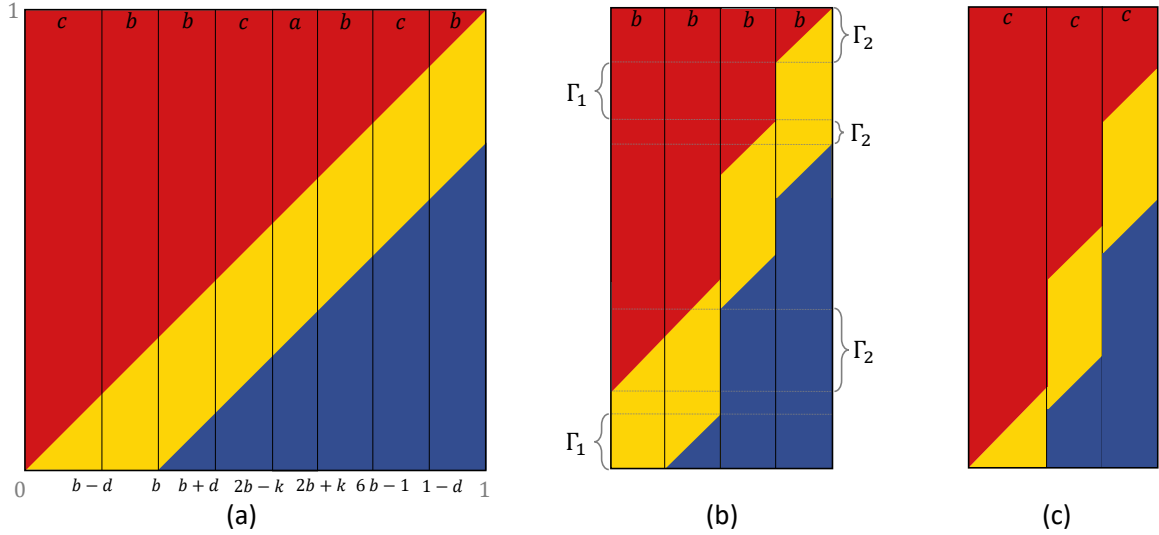
Figure 11: Construction for biased observer model
