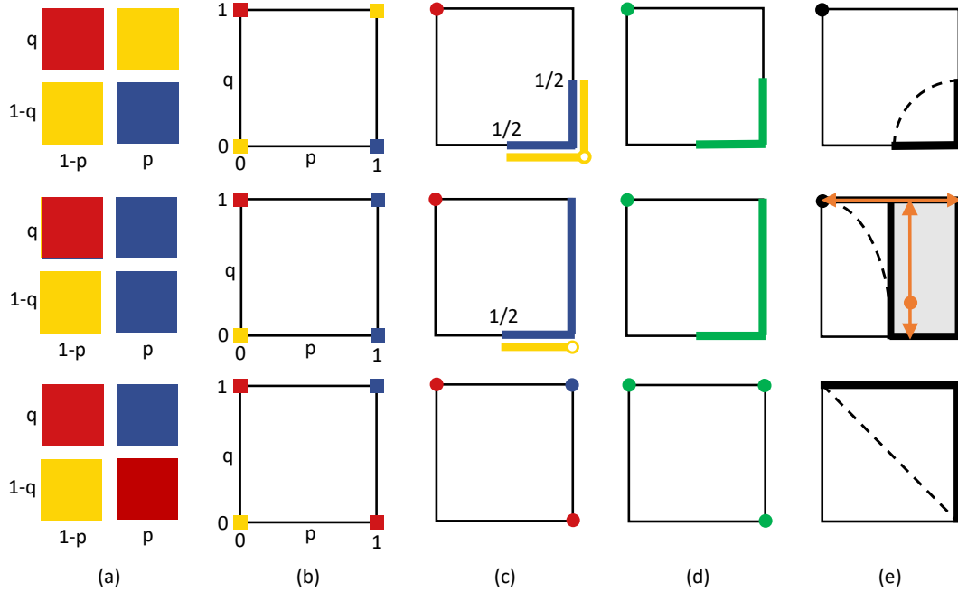
Figure 7: Biconvex hulls of subversive terminal beliefs
