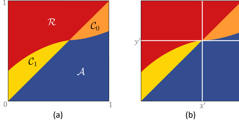
Figure 3: Uncertain direction of conflict
