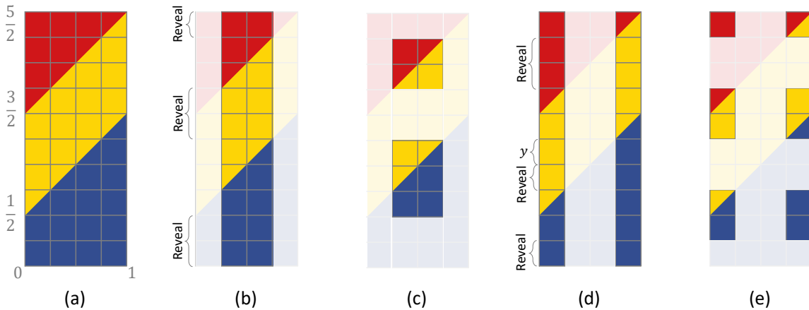
Figure 9: Recursive conversation for game \Gamma_\diamond
