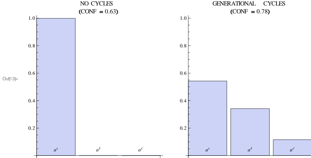
Figure 2: Asymptotic distribution of the population over the possible actions \{a^s, a^I, a^{s'}\} under two environments. CONF gives the equilibrium fraction of the population that faces internal conflicts.
